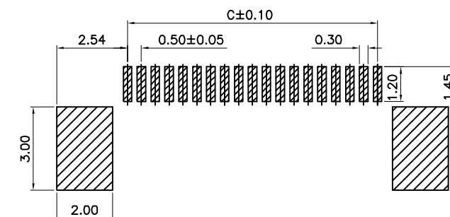
PCB Layout Reference
