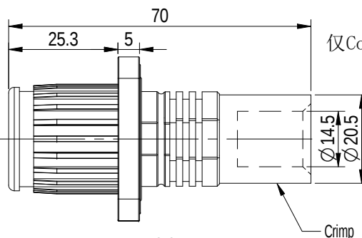
Crimp
