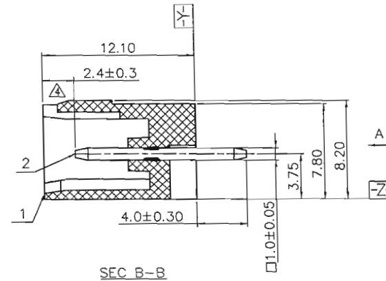
SEC B-B
