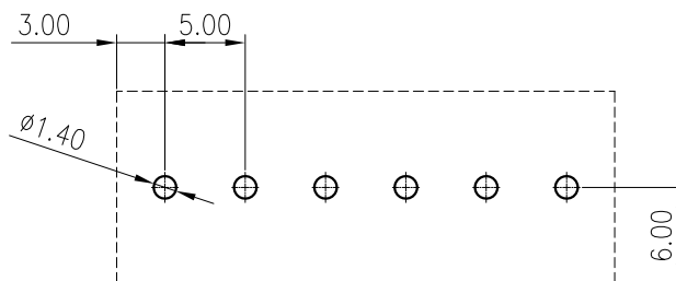
PCB LAYOUT
