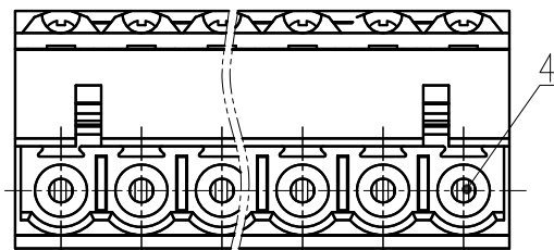
View A
