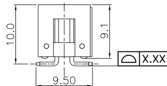
Coplanarity Information:
