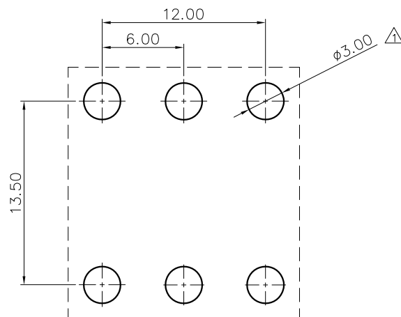
PCB LAYOUT
