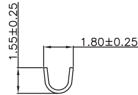
SEC B-B
