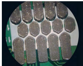
Solder paste as printed
