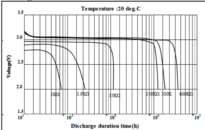
Discharge Characteristics
