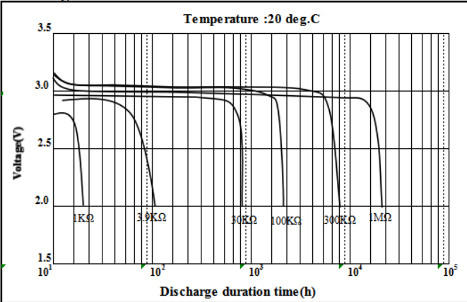
Discharge Characteristics
