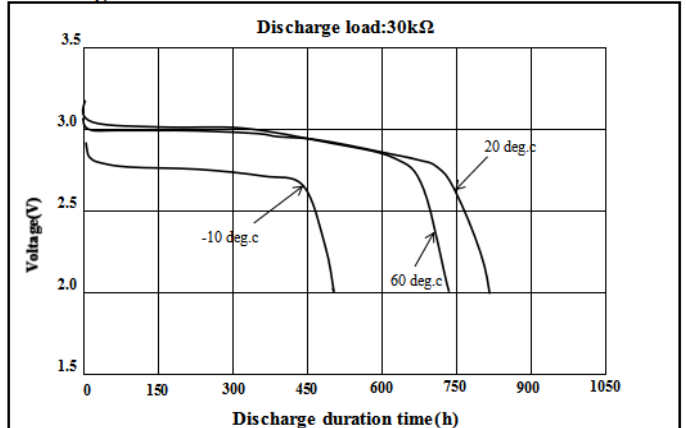
Discharge Characteristics
