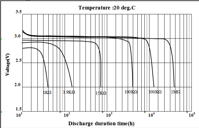
Discharge Characteristics
