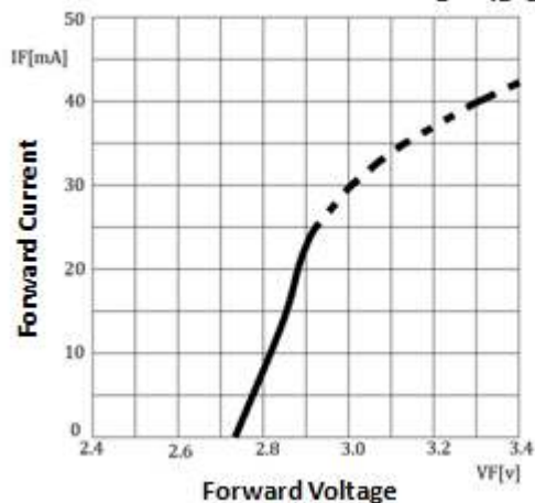
Forward Current vs Forward Voltage T_a = 25^\circ\text{C}
