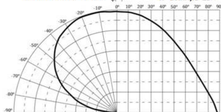
Radiation Characteristics I_F = 10\text{mA}, T_a = 25^\circ\text{C}
