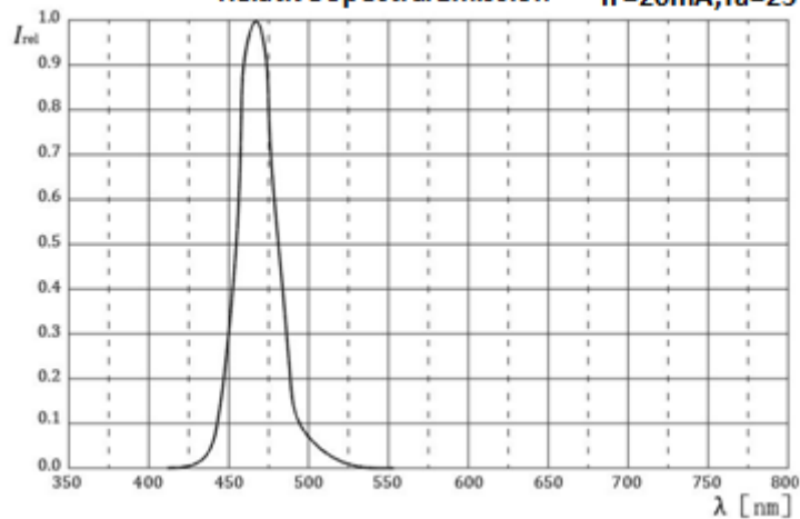
Relative Spectral Emission I_F = 20\text{mA}, T_a = 25^\circ\text{C}
