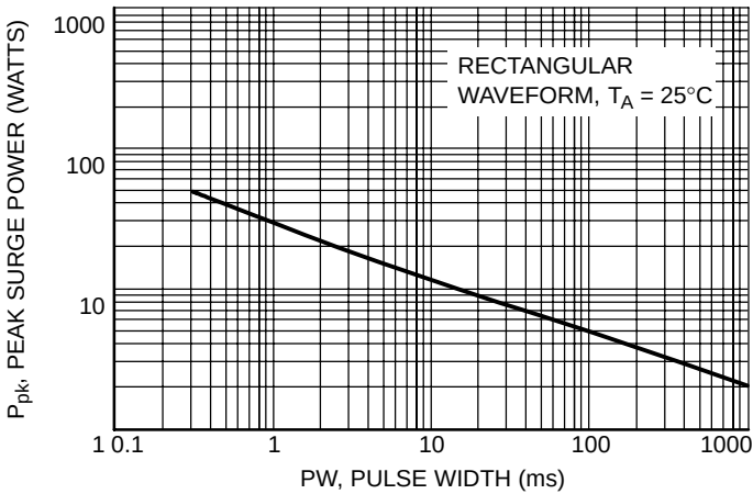
Fig.3 Maximum Nonrepetitive Surge Power
