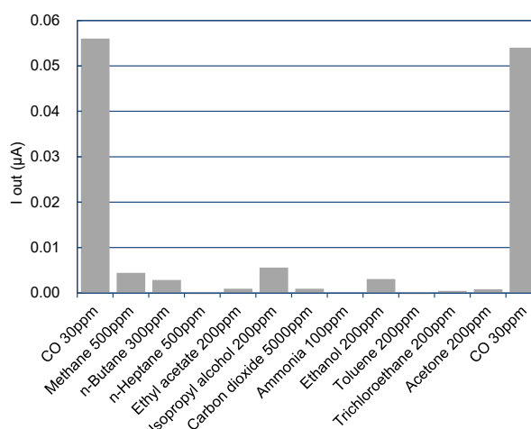
Figure 14a - Interference gas test (20°C/40%RH)
