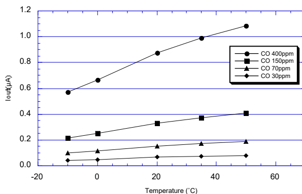
Figure 17a - Operation in high and low temperature (all data at 50%RH except test points)
