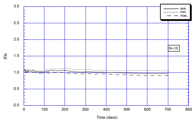
Figure 15 - Long term stability
