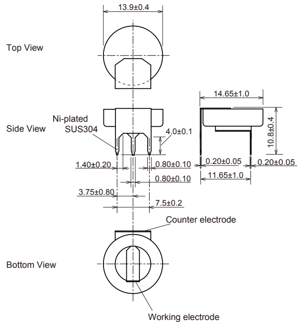
Figure 23 - Dimensions (w/lead pins) Unit : mm
