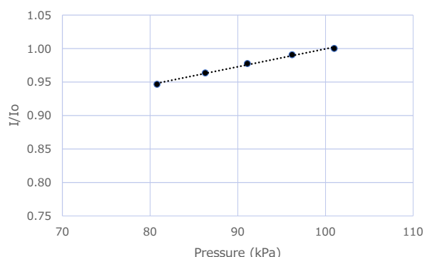
Fig. 13 - Pressure dependency
