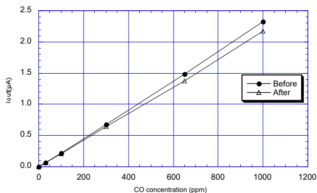
Figure 17b - Effects of shipping and storage
