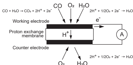
Figure 5 - Schematic diagram of TGS5141 operating principle
