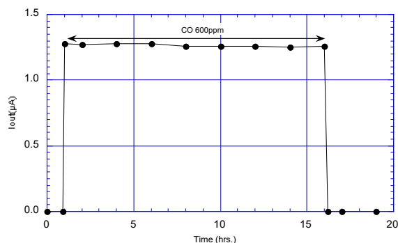
Figure 11a - Normal operation test (CO 600±30ppm for 12 hours at 20°C/40%RH)
