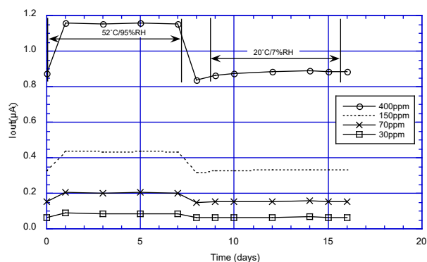
Figure 18a - Humidity test
