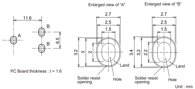
Figure 24 - Foot print example
