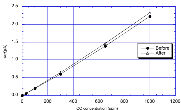
Figure 16 - Durability against corrosion
