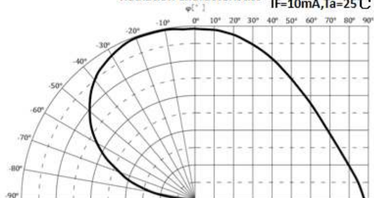
Radiation Characteristics
