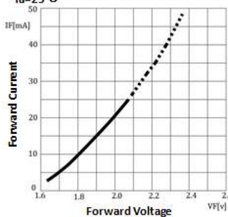
T_a = 25^\circ\text{C} Forward Current vs Forward Voltage
